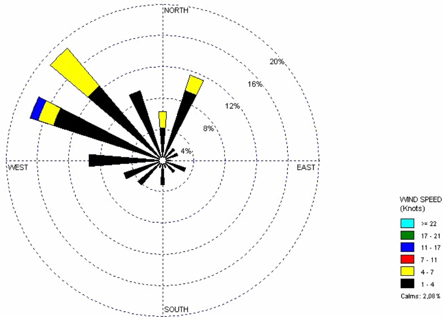
Figure 3b. Wind rose for the considered case base meteorological data
