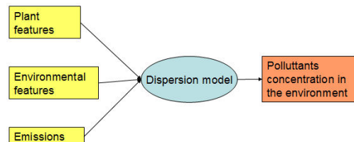
Figure 1. A schematic representation of the input-output of the adopted air dispersion model
