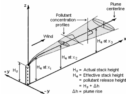
Figure 2. Schematization of the physical model on which AERMOD is based
