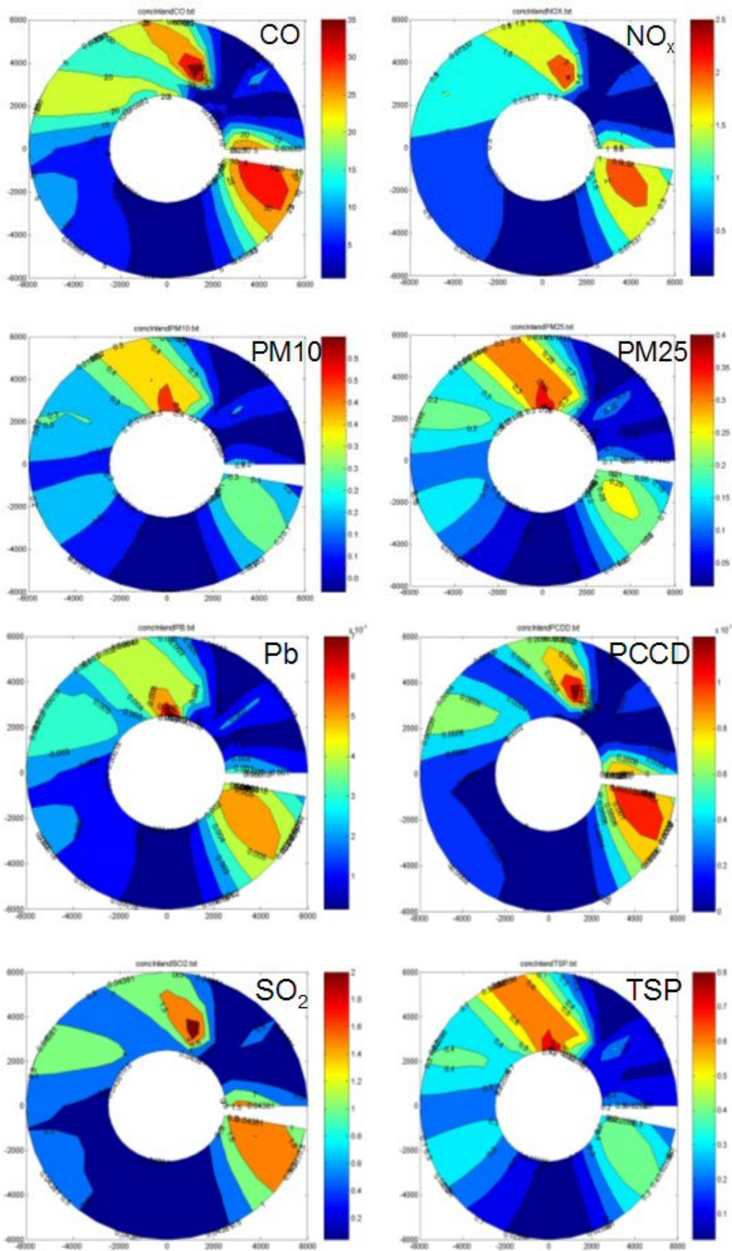
Figure 4a-h. The pictures show the results of the AERMOD simulation of air dispersion for the following pollutants (from left top to right bottom): CO, NO x , PM 10 , PM 25 , Pb, PCCD, SO 2 , TSP.
