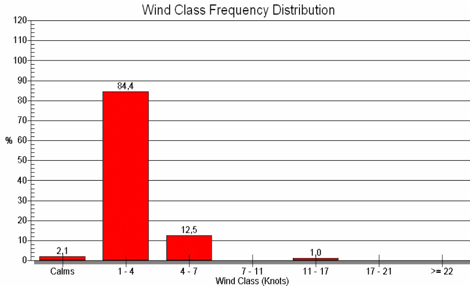
Figure 3a. Wind class frequency distribution for the case base
